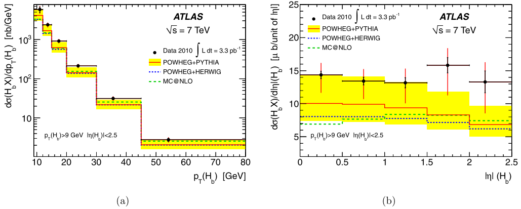
Fig. 3. Differential cross section for H_b production as a function of (a) p_T and (b) |\eta| of the b -hadron, in the fiducial kinematical region p_T(H_b) > 9 GeV, |\eta(H_b)| < 2.5 . The measurement is compared with the theoretical predictions, as described in the text. The inner error bars of the data points are statistical uncertainties, the outer are statistical + total systematic uncertainties.
