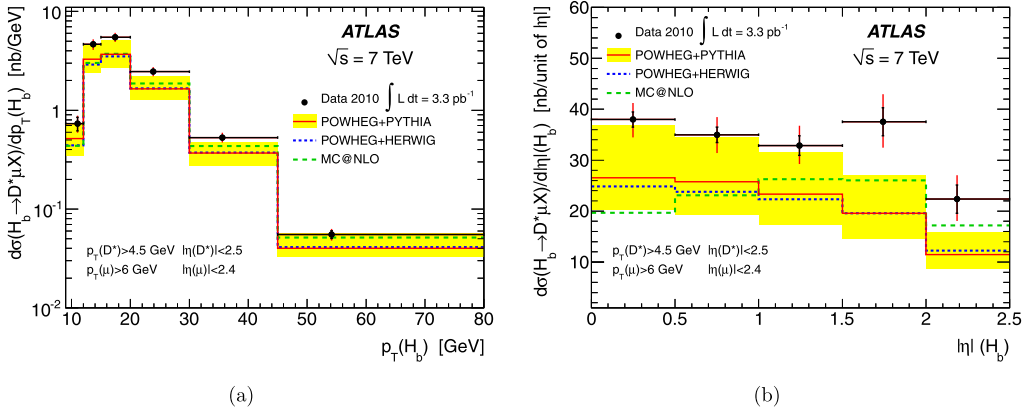
Fig. 2. Differential cross section for H_b \rightarrow D^{*+} \mu^- X production as a function of (a) p_T and (b) |\eta| of the b -hadron, in the fiducial kinematic region p_T(D^{*+}) > 4.5 GeV, p_T(\mu^-) > 6 GeV, |\eta(D^{*+})| < 2.5 and |\eta(\mu^-)| < 2.4 . The measurement is compared with the theoretical predictions, as described in the text. The inner error bars of the data points are statistical uncertainties, the outer are statistical + total systematic uncertainties.
