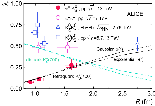
Fig. 4. The \lambda parameter as a function of source size R extracted from the \pi^\pm K_S^0 femtoscopic measurement in pp collisions at \sqrt{s} = 13 TeV. Results are compared with the previous ALICE measurements, obtained from K_S^0 K_S^0 [6,7] and \pi\pi [36] femtoscopic studies in pp and Pb-Pb collisions and the calculations from a toy geometric model (see text). The model calculations for the tetraquark and diquark hypotheses for the K_0^*(700) are shown as black and light green dashed lines, respectively, the short dashed lines representing the Gaussian \rho(r) and the long dashed lines representing the exponential \rho(r) .
