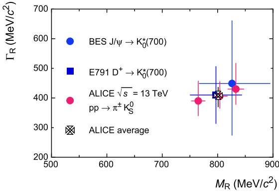
Fig. 3. The extracted Breit-Wigner parameters from the \pi^\pm K_S^0 femtoscopic correlation in pp collisions at \sqrt{s} = 13 TeV compared with those for K_0^*(700) from the BES [41] and the E791 [42] experiments. The horizontal and vertical bars represent the total uncertainties. The “ALICE average” value is the weighted average of the three ALICE points.
