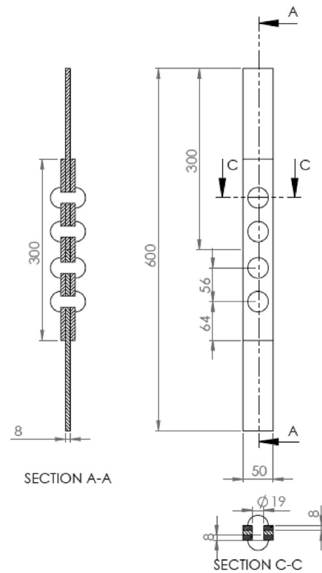
Fig. 2 – Single line double shear riveted (SLDSR) specimens [38].
