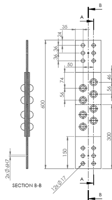
Fig. 3 – Double line double shear riveted (DLDSR) specimens [38].
