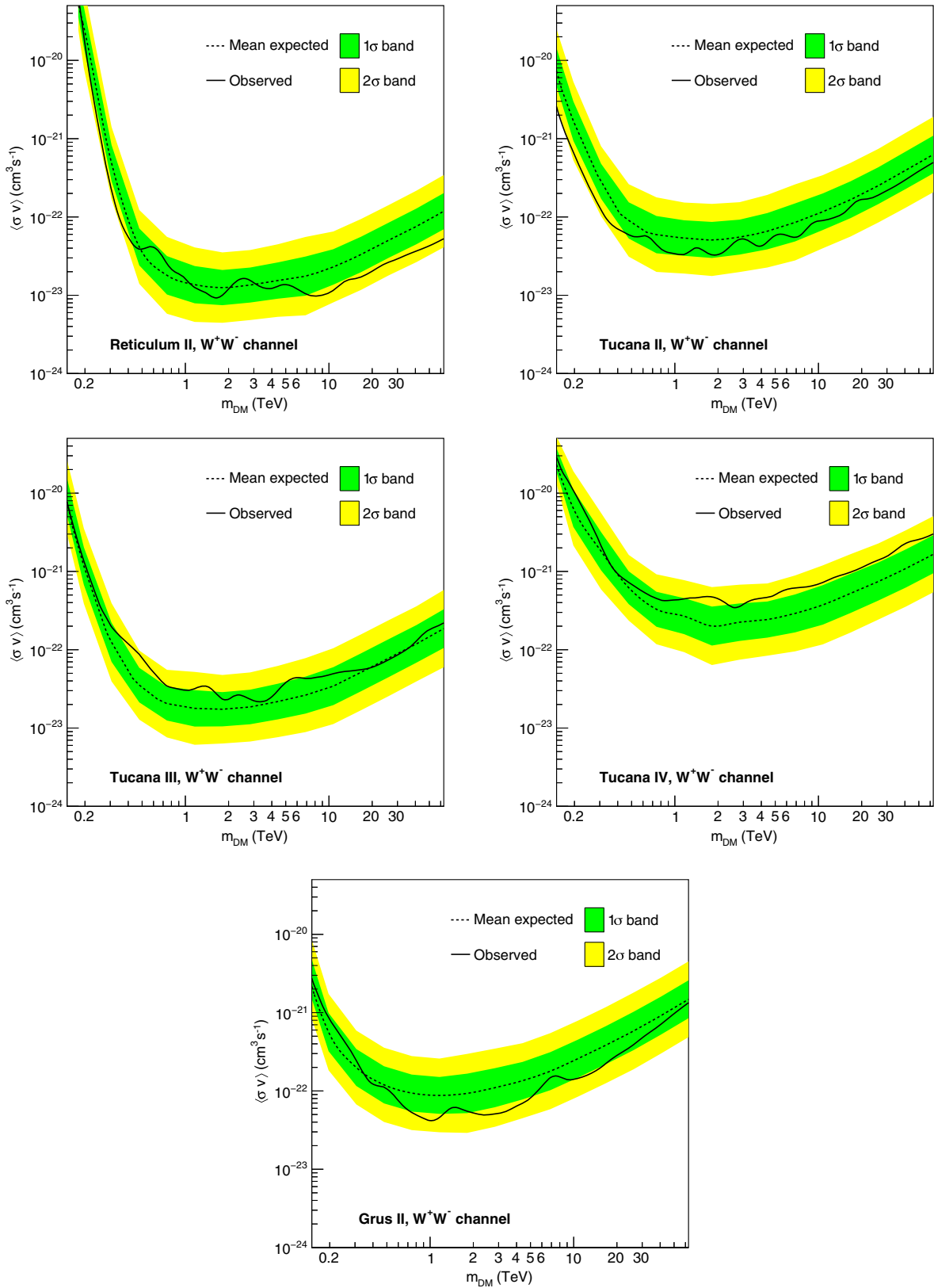
FIG. 2. 95% C.L. upper limits on the annihilation cross section \langle\sigma v\rangle for Ret II, Tuc II, Tuc III, Tuc IV, and Gru II, in the W^+W^- annihilation channel without the uncertainty on the J -factor. Observed limits (solid lines) together with mean expected limits (dashed line) and the 1\sigma (green area) and 2\sigma (yellow area) containment bands are shown.
