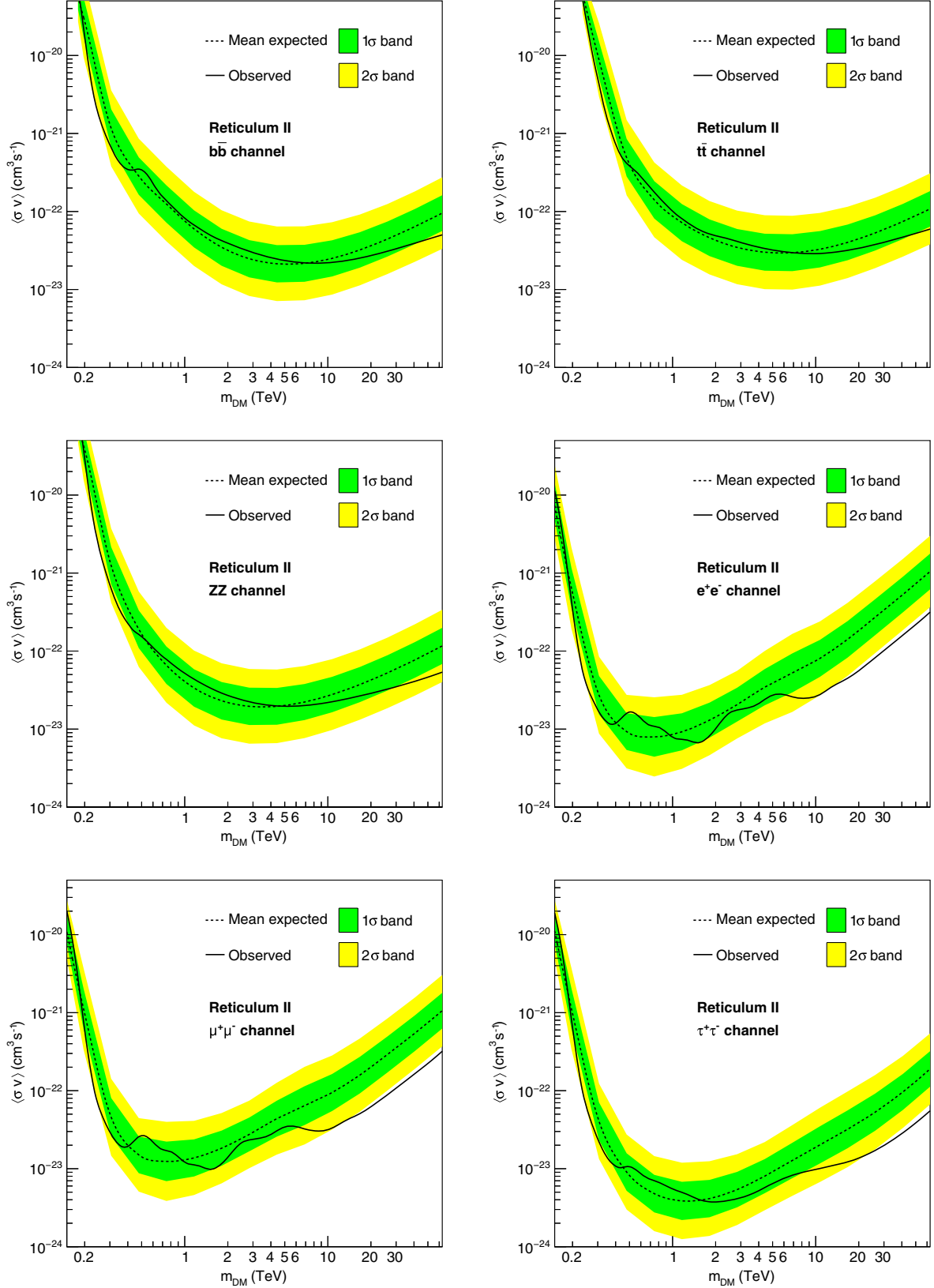
FIG. 4. 95% C.L. upper limits on the annihilation cross section \langle\sigma v\rangle for Ret II in the b\bar{b} , t\bar{t} , ZZ , e^+e^- , \mu^+\mu^- , \tau^+\tau^- annihilation channels, respectively, without the uncertainty on the J -factor. Observed limits (solid lines) together with mean expected limits (dashed lines) and the 1σ (green area) and 2σ (yellow area) containment bands are shown. The limits for the other targets can be found in Figs. 9–12 in the Appendix.
