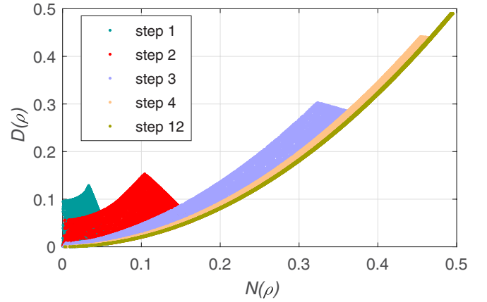
FIG. 13. Quantum discord D(\rho) vs negativity N(\rho) . Each surface with a different color shows the mean value of 10^4 random unitary matrices U_1 and control qubit initial states used to compute the quantum correlations for each purification step of the auxiliary qubit. Due to the similar behavior of the quantum correlations for the intermediate steps of the purification process, only 5 out of a total of 12 steps have been plotted.
