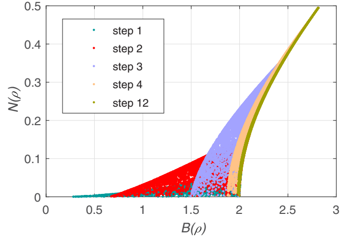
FIG. 9. Negativity N(\rho) vs B(\rho) . Each surface with a different color shows the mean value of 10^4 random unitary matrices U_1 and control qubit initial states used to compute the quantum correlations for each purification step of the auxiliary qubit. Due to the similar behavior of the quantum correlations for the intermediate steps of the purification process, only 5 out of a total of 12 steps have been plotted.
