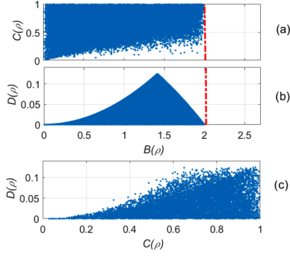
FIG. 2. Each dot represents the value of the quantum correlation calculated for the output state of the DQC1 circuit. The 10^6 states were obtained choosing initial states and unitary transformations at random. The red-dashed vertical line represents the maximum value of B(\rho) in which there is no Bell's nonlocality. The quantum correlation measured by entanglement does not appear here because it is null for the standard DQC1 circuit (see Fig. 1).
