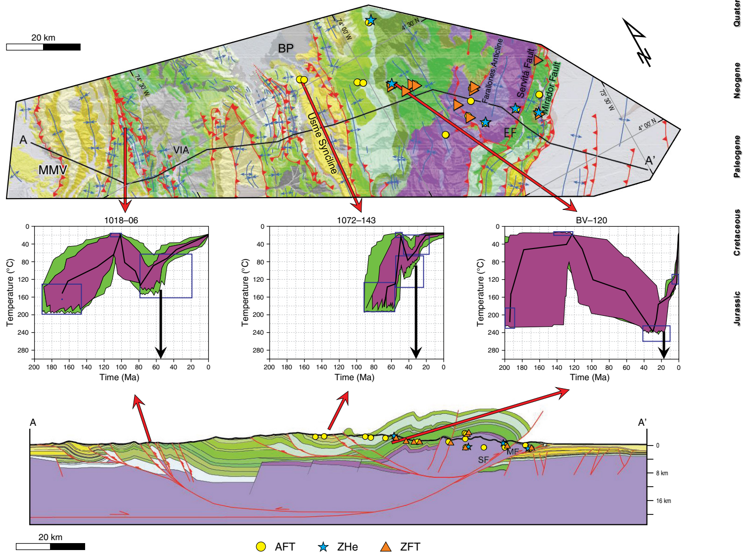
Figure 7. Geologic map (above) and structural cross section (below) at the latitude of Bogotá (4° N, after Mora et al., 2015) showing geologic context for three representative 1D thermal models constructed using multiple thermochronometers with HeFTy software (Ketcham, 2005). The time-temperature (t-T) paths show good (purple) and acceptable (green) thermal histories that fit the observed data. (MMV) Middle Magdalena Basin; (VIA) Villeta Anticlinorium; (BP) Bogotá Plateau; (EF) Eastern Foothills.
