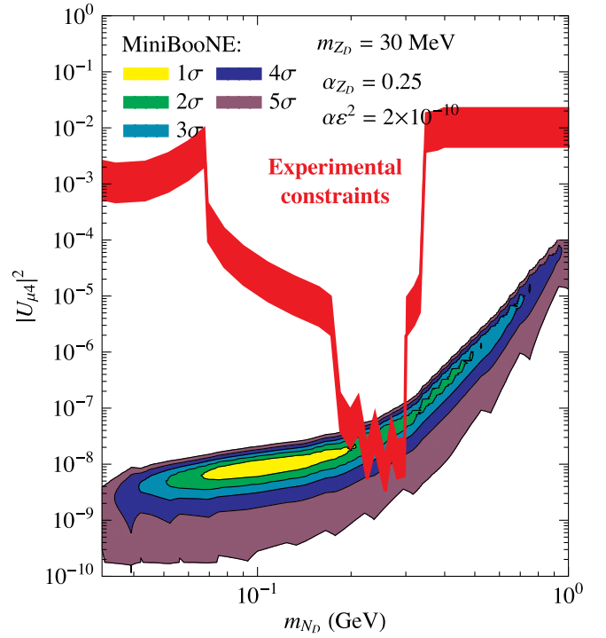
FIG. 3. Region of our model in the |U_{\mu 4}|^2 versus m_{N_D} plane satisfying MiniBooNE data at 1\sigma to 5\sigma C.L., for the hypothesis m_{Z_D} = 30 MeV, \alpha_{Z_D} = 0.25 , and \alpha \epsilon^2 = 2 \times 10^{-10} . The region above the red curve is excluded at 99% C.L. by meson decays, the muon decay Michel spectrum and lepton universality [35,36].
