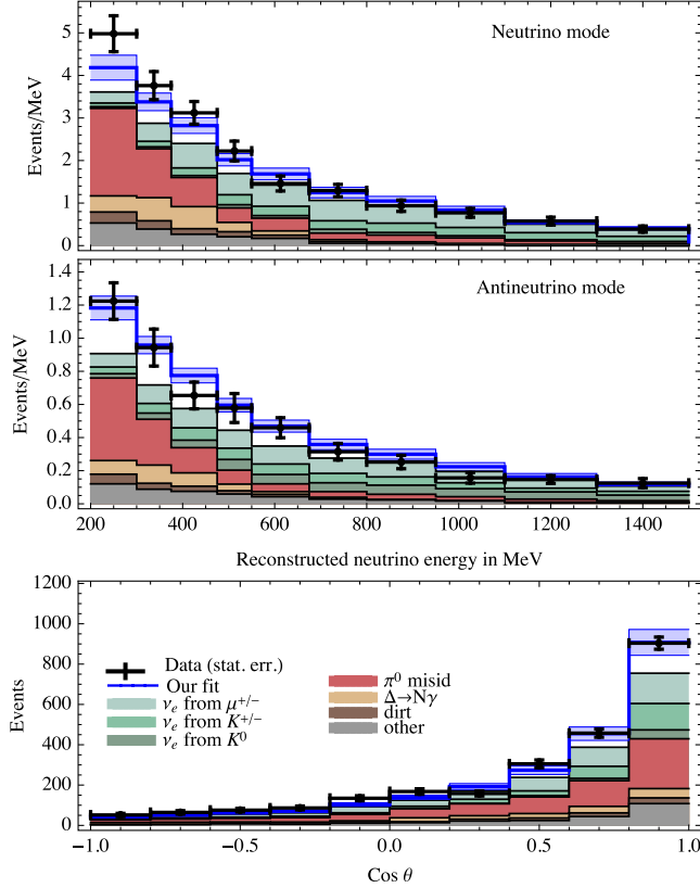
FIG. 2. The MiniBooNE electronlike event data [18] in the neutrino (top panel) and antineutrino (middle panel) modes as a function of E_\nu^{\text{rec}} , as well as the \cos \theta distribution (bottom panel) for the neutrino data. Note that the data points have only statistical uncertainties, while the systematic uncertainties from the background are encoded in the light blue band. The predictions of our benchmark point m_{N_D} = 420 MeV, m_{Z_D} = 30 MeV, |U_{\mu 4}|^2 = 9 \times 10^{-7} , \alpha_{Z_D} = 0.25 , and \alpha \epsilon^2 = 2 \times 10^{-10} are also shown as the blue lines.
