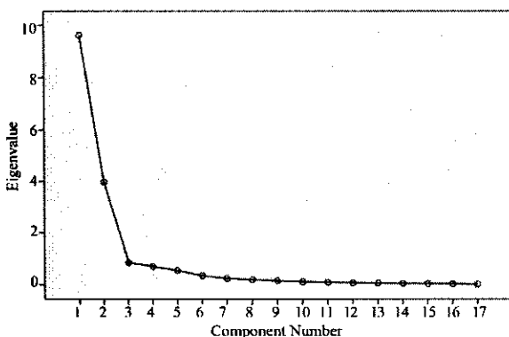
Figure 2. Scree plot.
