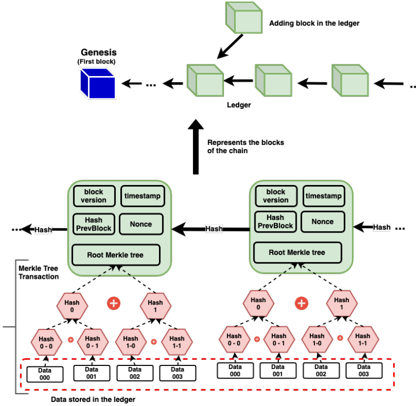
Fig. 2. The primary blockchain structure, adapted from [36, 103]. Figure shows the way the ledger is structured in blockchain networks and describes the components that are inside the distributed ledger. The genesis block is assigned automatically when the network is started, with hash default values, and other blocks are inserted in ledger following the genesis. In block structures, one could include components such as hash from the previous block, nonce, timestamp, block version, and the value known as the root of the Merkle tree. The Merkle tree is used to organize transactions into a blockchain network, and store them with security, as shown in the red line. The attributes allocated into the block, could be modified depending on the consensus protocol used; in summary, this figure presents the characteristics inserted in blockchain structure like Ethereum and Bitcoin implementations.
