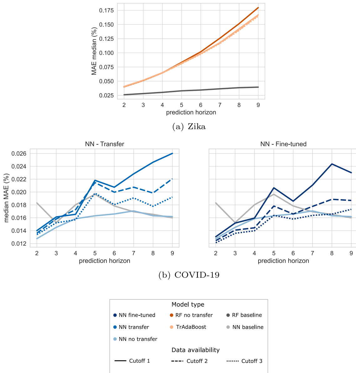
Fig. 5. Percent mean absolute errors for different prediction horizons and model types within the best-performing algorithm of each disease.
