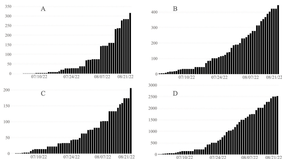
Fig. 2. Epidemic curve of the four analyzed states: GO-FD (A), RJ (B), MG (C) and SP (D).
