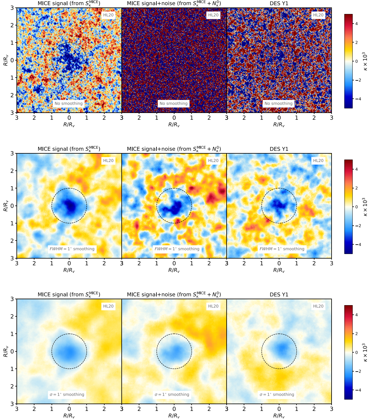
Figure 2. Simulated signal-only stacked \kappa images from MICE (left-hand panels) in comparison to noise-added versions (centre panels) and observed DES Y1 stacked results (right-hand panels) for the HL20 version of 2D voids. All versions of our results are displayed, without smoothing (top panels) and with \text{FWHM} = 1^\circ (middle) or \sigma = 1^\circ (bottom panels) Gaussian smoothings are used. The re-scaled void radius R/R_v = 1 is marked by the dashed circles. We identify important trends with changing smoothing scales but overall report good consistency between data and simulations.
