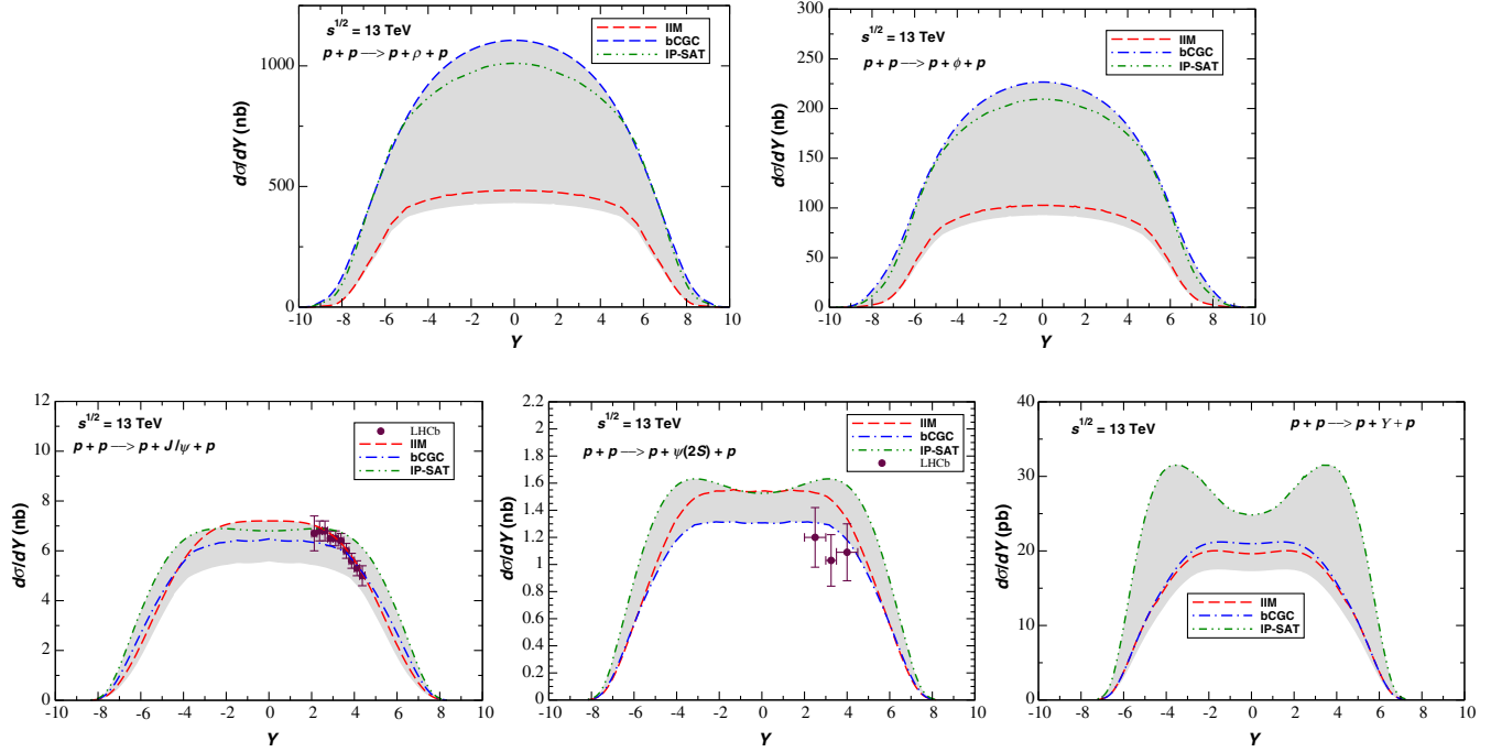
FIG. 4. Rapidity distributions for exclusive photoproduction of \rho , \phi , J/\psi , \psi(2S) and Y in pp collisions at \sqrt{s} = 13 TeV. Data is from the LHCb Collaboration [31–33].
