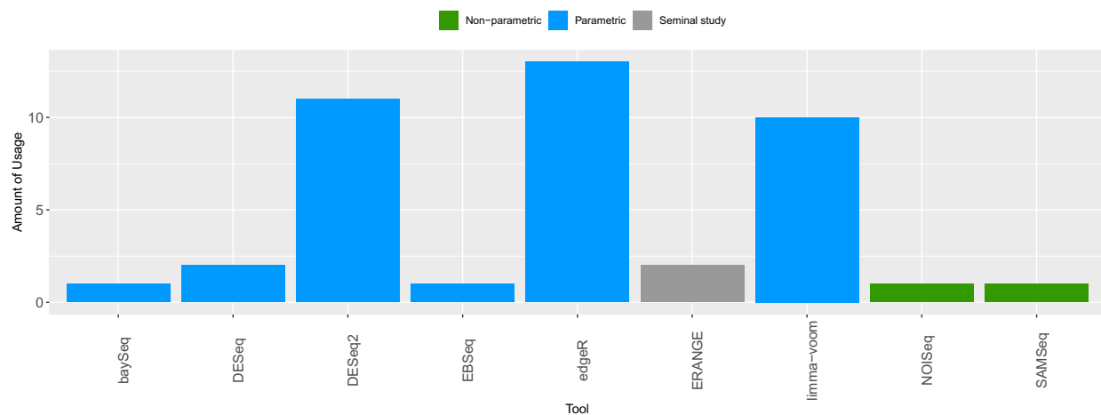
Fig. 4. Histogram of the use of the methods: The X-axis presents only the tools used as a base (dependency) for some other tool. The bars are colored according to the category of the tool, following the identification colors of the timeline (Fig. 2) and the interaction network (Fig. 3), where blue shows parametric methods, green non-parametric and gray “seminal studies”. The items that contain * in the name indicate tools developed in the context of single-cell sequencing analysis.
