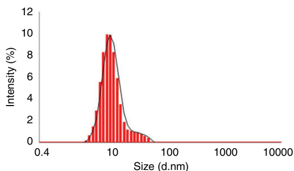
Figure 2. Particle size distribution of CG-CuNPs by DLS.
