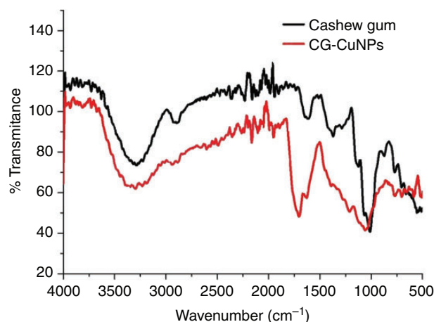
Figure 4. ATR-FTIR spectra of cashew gum and CG-CuNPs.
