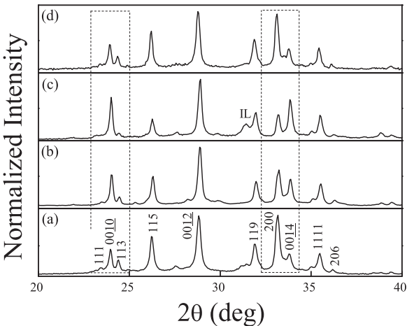
Fig. 1. The X-ray diffraction patterns of the powdered ST5 sample (a), and of bulk samples SP5 (b), ST5 (c) and REF (d). The X-ray data of the pellets were taken on the surface perpendicular to the compacting pressure direction. The reflections belonging to the Bi-2223 phase are marked by Miller indexes in (a). Selected regions of the diagrams, marked as dashed boxes, are discussed in the text.
