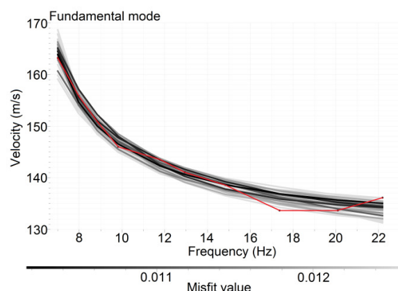
Figure 7. Comparison among the experimental (from the seismograms acquired using weight drop source) and numerical dispersion curves obtained from the models. The darker lines indicate the lowest misfits.
