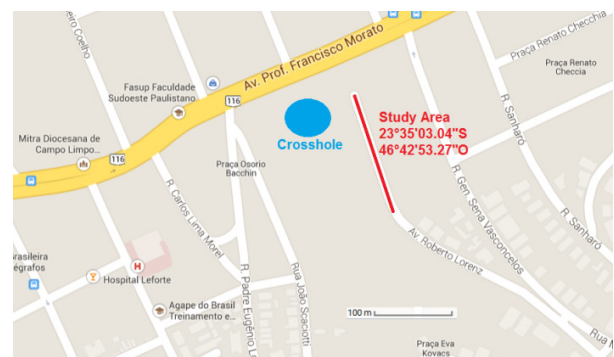
Figure 1. Map showing the studied area with location of the MASW test (redline) and the crosshole test (blue oval-shaped area). Google Maps, 03/11/2015.
