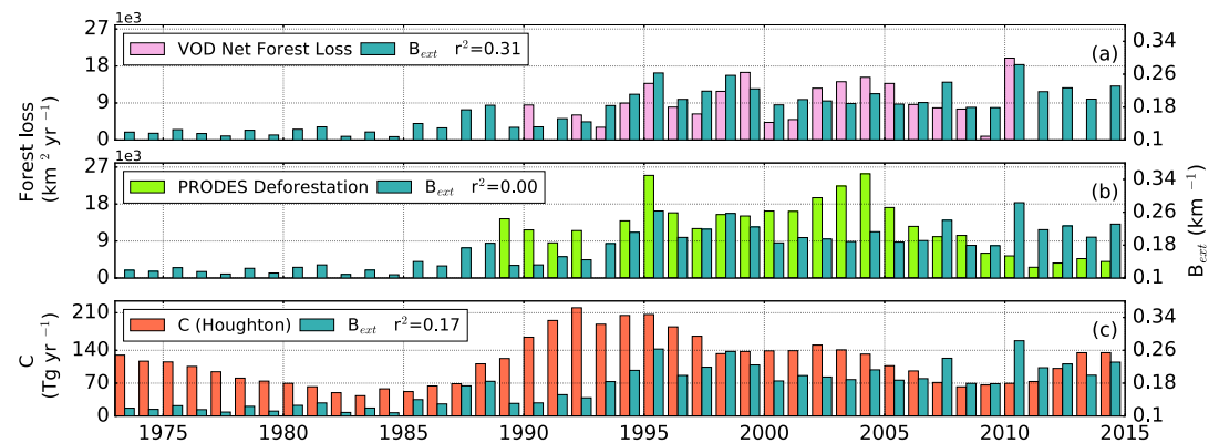
Figure 8. Annual estimates of fire emissions and forest loss for the whole study region (Figure 2). In all plots dark green indicates the annual averaged visibility-based B_{\text{ext}} (1974–2014), which are compared with (a) VOD-based net forest loss (1990–2010), (b) summed PRODES deforestation for the provinces of Acre, Mato Grosso, Rondônia, Pará, and Tocantins (1989–2014), and (c) averaged FAO emissions attributed to deforestation fires for Brazil and Bolivia.
