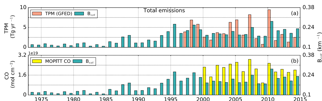
Figure 4. Averaged B_{\text{ext}} values for the whole study region [7°S–17°S, 48°W–68°W], compared with (a) GFED-based TPM emissions (1997–2014) and (b) MOPITT CO concentrations (2000–2014) for the same region.
