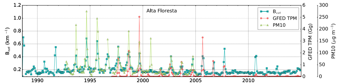
Figure 5. Monthly averaged B_{ext} and ground-based measurements of PM_{10} , both observed at Alta Floresta, and averaged GFED TPM emissions for the 36\ 0.25^\circ \times 0.25^\circ grid cells centered over Alta Floresta.
