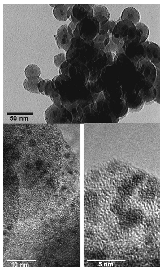
Figure 3. TEM analysis of the spent Ir 0 catalyst.
