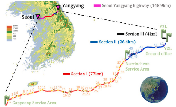
Fig. 6. Measurement campaign sections and tunnels. The trip was divided into three sections (I, II, and III). Section 1 (red line) is from Gapyeong service area to Naerinceon service area and Section 2 (blue line) is to Y2L ground office. Section 3 (black line) is on a local road from Y2L ground office to Y2L underground lab. Tunnels are numbered in sequence. The specification of each tunnel can be found in Table 2.
