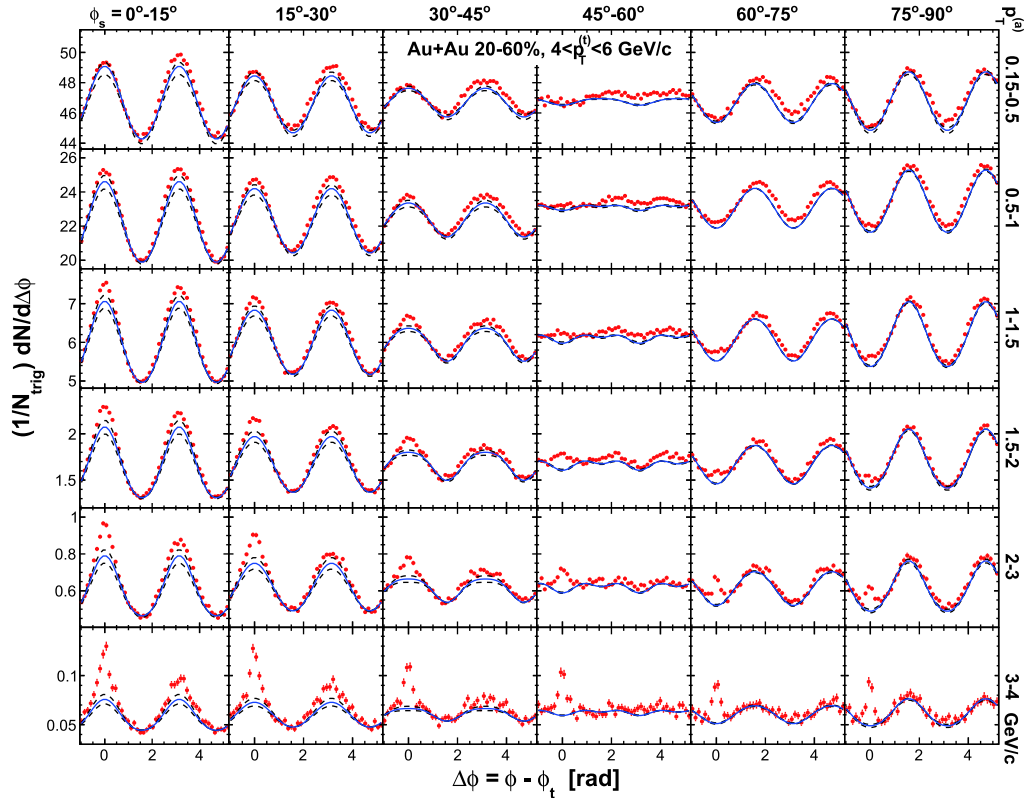
Fig. C2. (color online) Same as in Fig. C1 but for trigger particle 4 < p_T^{(t)} < 6 GeV/c and six bins in associated particle p_T^{(a)} .
