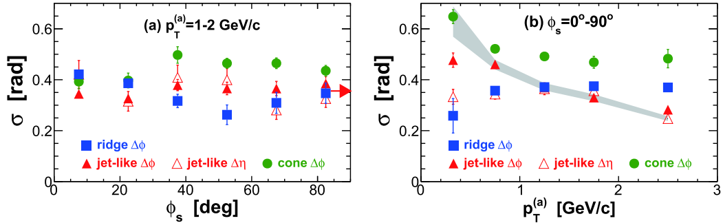
Fig. 19. (color online) Fit Gaussian widths of the near-side jet-like correlation, the near-side ridge, and the away-side double-peak: (a) as a function of \phi_s = |\phi_t - \psi_{EP}| for 1 < p_T^{(a)} < 2 GeV/c, and (b) as a function of p_T^{(a)} for the \phi_s -integrated correlation. The \Delta\eta Gaussian width for the jet-like correlation is also shown. Data are from 20%-60% Au+Au collisions. The trigger p_T^{(i)} range is 3 < p_T^{(i)} < 4 GeV/c. Error bars are statistical only. The near-side jet-like \Delta\phi correlation Gaussian width from the minimum bias d +Au data is indicated by the arrow in (a) and by the shaded area in (b); the width of the shaded area indicates the statistical uncertainty.
