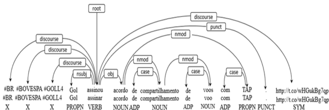
FIGURE 1 – Example of UD-annotated tweet from the DANTEStocks.
