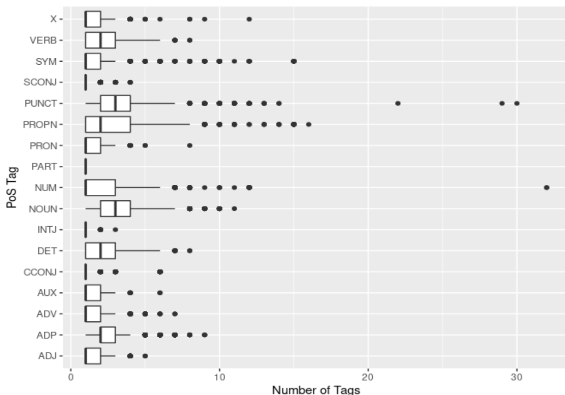
FIGURE 3 – PoS tags frequency inside the tweets where they occur.
