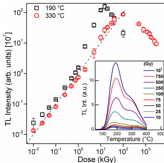
Fig. 4. TL response curves as functions of radiation dose for pink tourmaline. In the inset are presented the TL glow curves of pink tourmaline irradiated with 10, 25, 50, 75, 100, 250, 500, 750 and 1000 Gy of \gamma -rays. (For interpretation of the references to color in this figure legend, the reader is referred to the web version of this article.)
