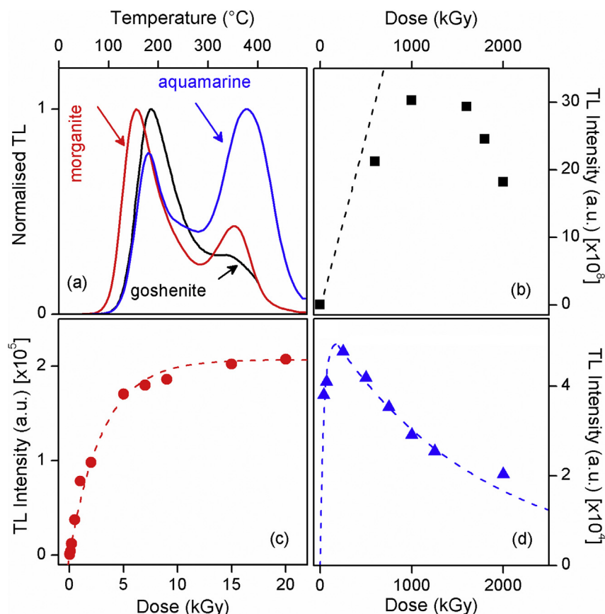
Fig. 3. (a) TL glow curves of morganite, goshenite and aquamarine and TL response curves as functions of radiation dose of (b) goshenite, (c) morganite and (d) aquamarine.
