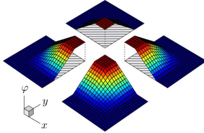
Figure 2. 2D Flat-Top PU components on quadrilateral finite elements. Adapted from Ramos [14].
