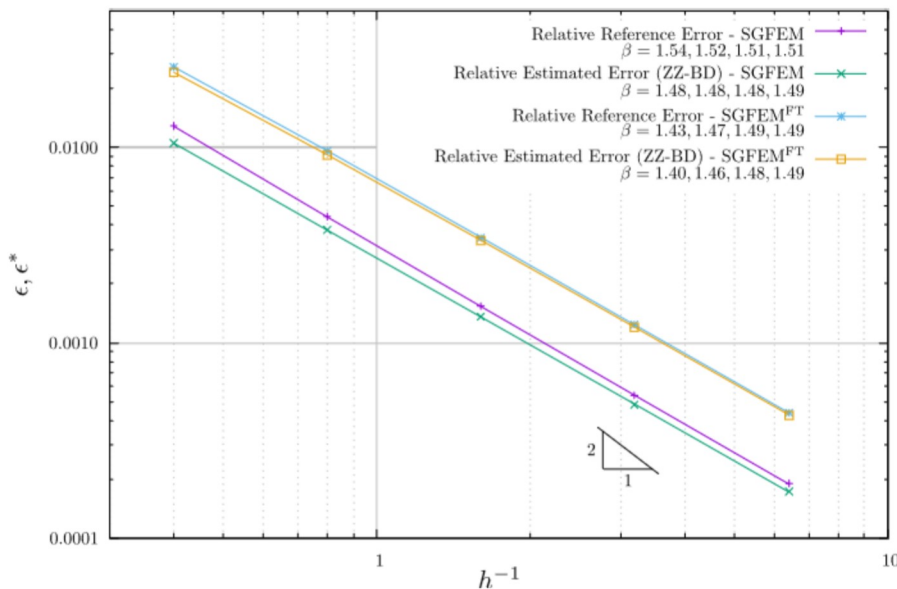
Figure 4. Error convergence in energy norm for SGFEM and SGFEM FT .
