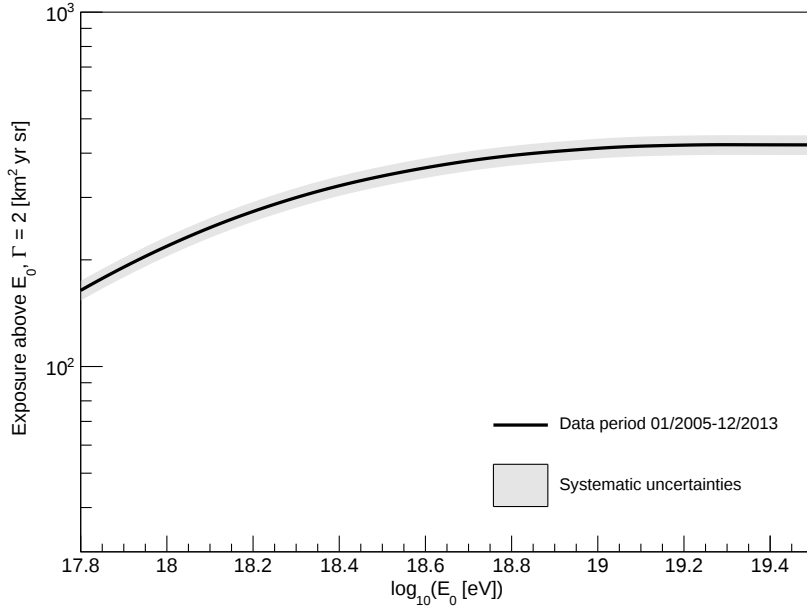
Figure 1. Hybrid exposure for primary photons in the time interval 1 January 2005–31 December 2013, assuming a power-law spectrum with \Gamma = 2 . Systematic uncertainties due to the ontime and the trigger efficiency are shown as a gray band.
