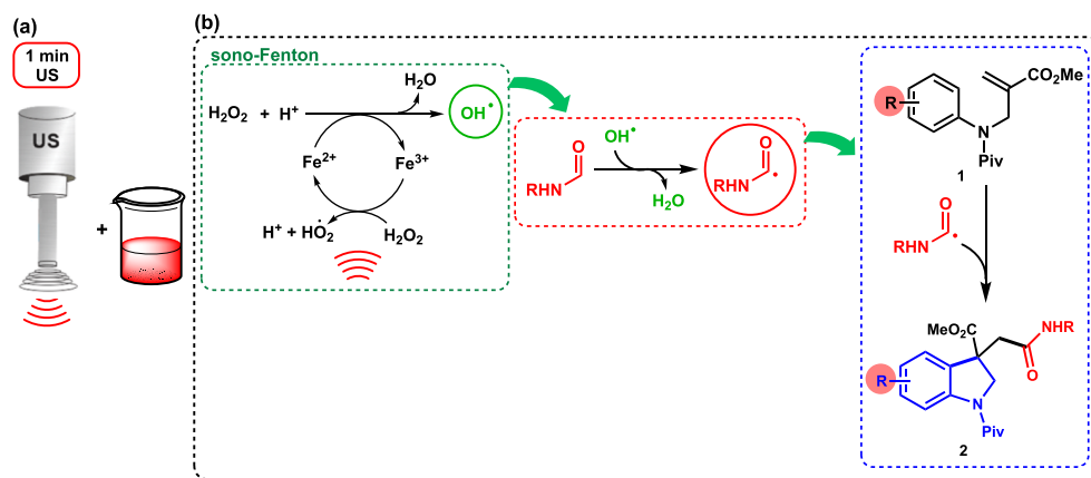
Fig. 3. Combining ultrasound and the Fenton reaction in formamide for fast indoline construction. (a) Experimental setup; (b) Sequence of radical reactions: hydroxyl radical generation, carbamoyl radical generation and indoline formation.
