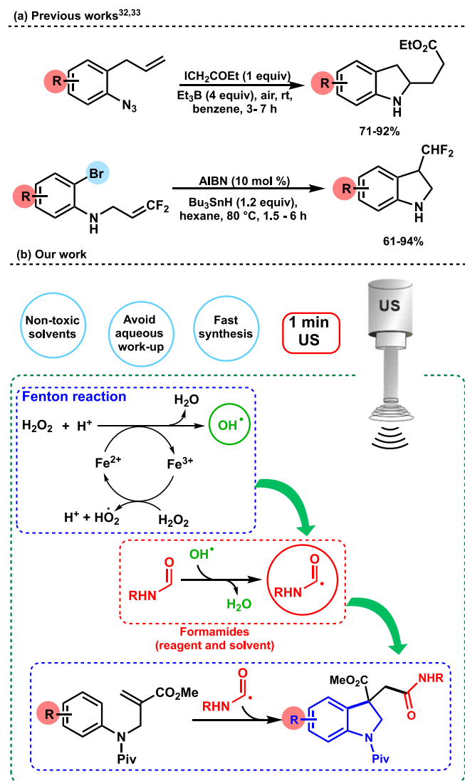
Fig. 2. (a) Previous works involving radical cascade reactions for synthesis of indolines (b) Our work: a fast approach enabled by ultrasonic irradiation to construct novel functionalized indolines.
