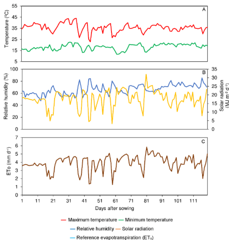
Figure 1. Meteorological variables.
