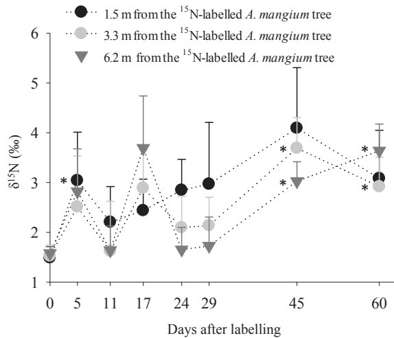
Fig. 6. \delta^{15}\text{N} values over the 60 day period of young leaves of Eucalyptus grandis pairs located at a distance of 1.5 m, 3.3 m and 6.2 m from the ^{15}\text{N} -labeled Acacia mangium . The background values are indicated for the labeling date (day 0). Vertical bars indicate standard errors between blocks ( n = 3 ). At a given collection date and a given distance, * indicates significant differences with \delta^{15}\text{N} background values ( P < 0.05 ). The mean background \delta^{15}\text{N} values \pm standard error ( n = 3 ) were 1.49 \pm 0.36\text{‰} , 1.53 \pm 0.35\text{‰} , and 1.58 \pm 0.21\text{‰} , at a distance of 1.5 m, 3.3 m and 6.2 m, respectively.
