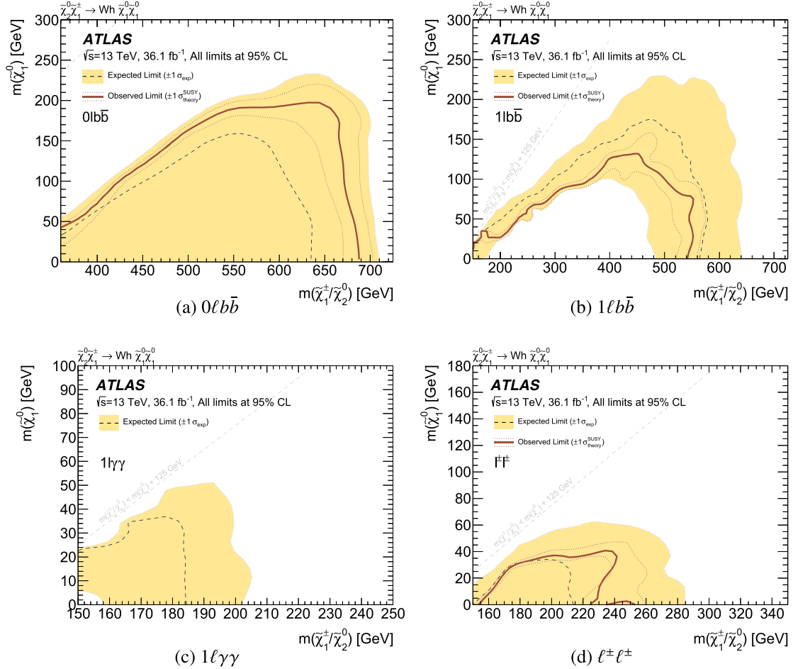
FIG. 12. The expected and observed exclusion for the 0\ell b\bar{b} , 1\ell b\bar{b} , 1\ell\gamma\gamma , and \ell^\pm\ell^\pm channels. Experimental and theoretical systematic uncertainties, as described in Sec. VII, are applied to background and signal samples and illustrated by the yellow band and the red dotted contour lines, respectively. The red dotted lines indicate the \pm 1 standard-deviation variation on the observed exclusion limit due to theoretical uncertainties in the signal cross section.
