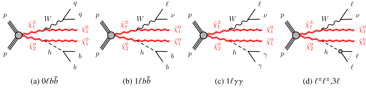
FIG. 1. Diagrams illustrating the signal scenarios considered for the pair production of chargino and next-to-lightest neutralino targeted by the (a) hadronic ( 0\ell b\bar{b} ) and (b) 1\ell b\bar{b} , (c) 1\ell\gamma\gamma , (d) \ell^\pm\ell^\pm, 3\ell leptonic channel selections. In (a) and (b) the Higgs boson decays into two b -quarks. In (c), the diphoton channel is shown with h \rightarrow \gamma\gamma . In (d), the visible multilepton final state of the Higgs boson is shown. Leptons are either electrons or muons.
